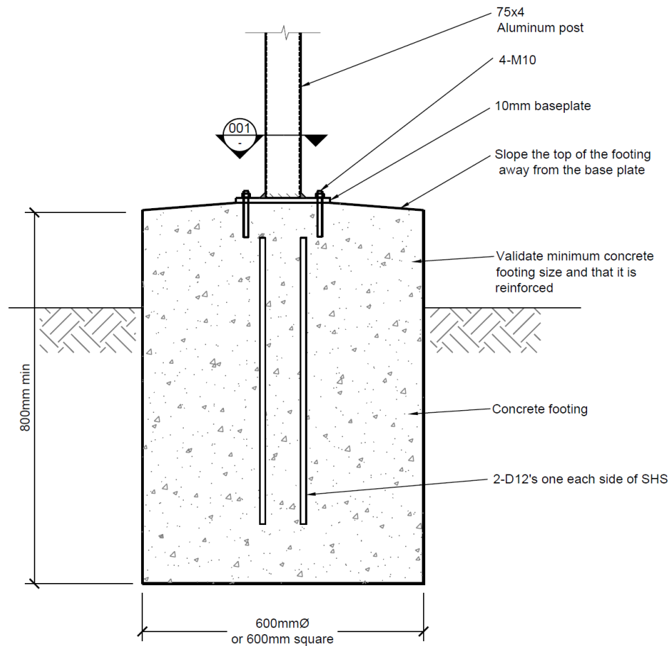
1 POST TO CONCRETE FOOTING SCALE 1:10
